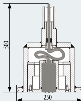
Tank installation
