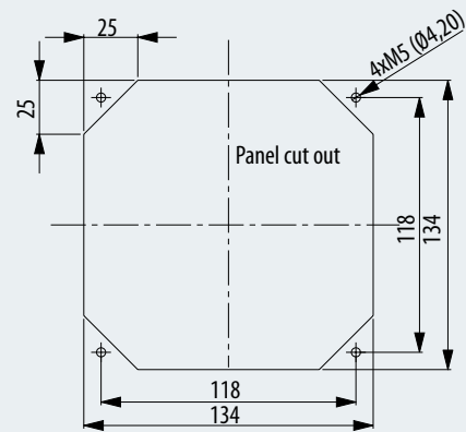
Display panel cut out
