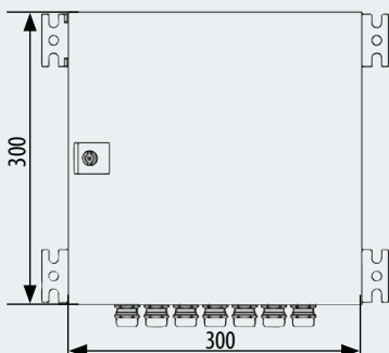
Electronic unit
