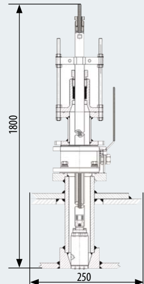
DB gate valve
