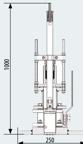
SB gate valve
